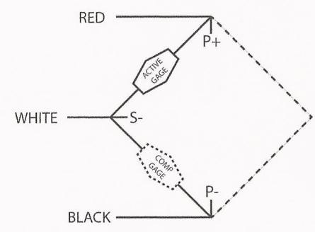
WIRING DIAGRAM
