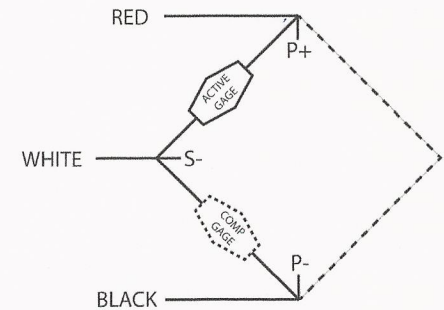
WIRING DIAGRAM
