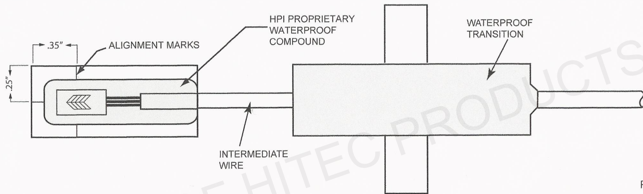
WIRING DIAGRAM
