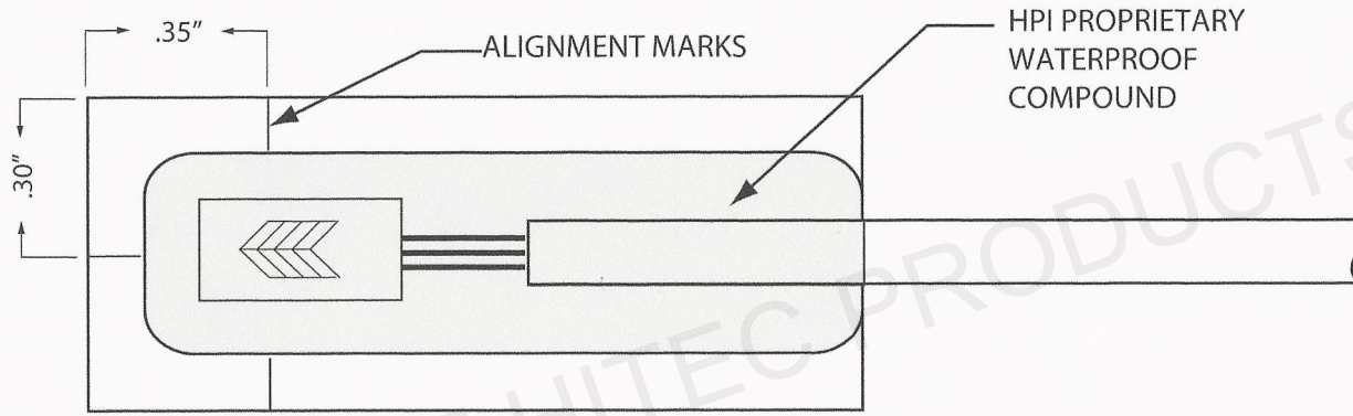
WIRING DIAGRAM
