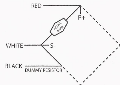
WIRING DIAGRAM x 3
