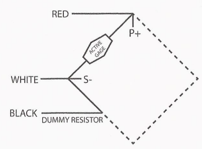
WIRING DIAGRAM x 3
