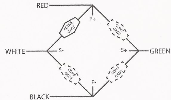
WIRING DIAGRAM x 3
