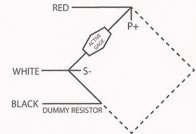
WIRING DIAGRAM x 2
