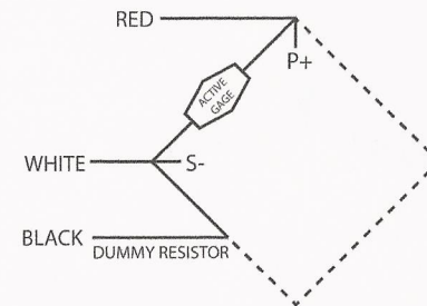
WIRING DIAGRAM x 2
