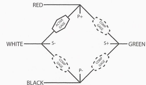
WIRING DIAGRAM
